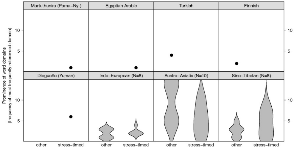
Figure 1: Strength of evidence for prosodic words plotted against rhythm classifications. Panel 1–5: individual languages, panel 6–8: language families
