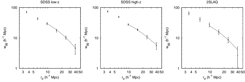
Figure 8. The projected galaxy–galaxy correlation functions w_{\text{gg}}(r_p) for the three samples and the best-fitting non-linear power spectrum (using the Smith et al. 2003 mapping) to the 7.5\text{--}47 h^{-1} \text{Mpc} . Note that the error bars are correlated.
