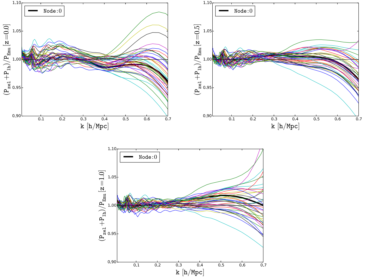
Figure 5. The residuals of our P(k) = P_{\text{Zel}}(k) + P_{1h}(k) expression against simulations for 38 different cosmological models (different colour curves in each panel) for three different redshifts.
