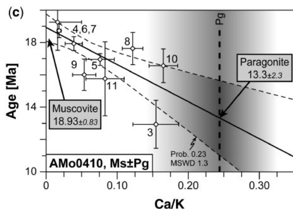
Fig. 10. Ar isotope results from Molare. (a) Age spectra for muscovite and (b) biotite from AMo0409 and AMo0410. (c) Ca/K vs age correlation diagram in muscovite–paragonite mixture AMo0410. Extrapolation toward the Ca/K value in paragonite directly determined by EMP (grey field, 0.25 \pm 0.09 ) yields the age of the pure paragonite. Error envelope is given as 2\sigma .
