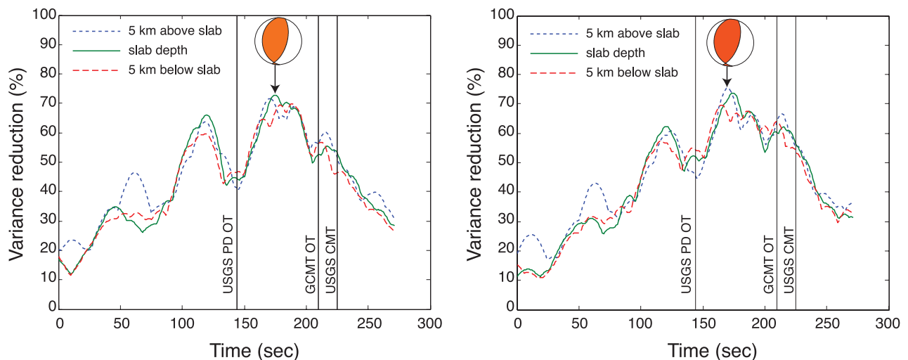
Figure 4. Temporal evolution of the maximum variance reductions for the velocity (left-hand panel) and acceleration (right-hand panel) inversions over the grid. The beach-balls show the best solutions (Fig. 3). Inversions start at time 05:44:02 UTC (0 s) and run for about 4.5 min, every second.
