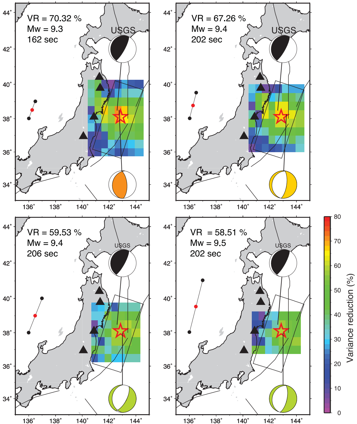
Figure 8. Effect of the increasing length of the QFS GFs on the GRiD MT capability to detect the M9 Tohoku earthquake. The QFS GFs are built using three point sources (black and red dots) and the moment tensor analysis is performed using the position of the centre point (red dots), every 0.5^\circ in latitude and longitude.
