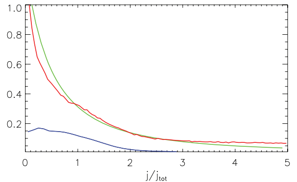
Figure 8. The final distribution of j = rV_c(r) for ‘observable’ baryons in the simulation, which consists of stars and H I gas (blue). In red we plot the distribution of all baryons which would have ended in the galaxy if outflows were not present, i.e. it is the distribution of stars, H I gas and warm/hot gas within the virial radius at z = 0 , combined with outflows whose angular momentum is determined at the time-step prior to being heated and expelled. An analytic fit, as determined in Bullock et al. (2001), to the typical distribution for dark matter haloes is overplotted (green).
