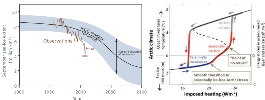
Fig. 9 Left Observed decline in September Arctic sea-ice cover (red line, in million square kilometers; solid line indicates satellite observations). The year 2007 showed an anomalously strong reduction of 23% compared to the previous record in 2005. Sea-ice extent recovered somewhat in 2008 and 2009, but reduced again in 2010. IPCC model simulations of 2007 (shading) strongly underestimated (currently observed) sea-ice decline (after Stroeve et al. 2007). Right Evolution of Arctic sea ice in response to warming simulated with an idealized physical model (Eisenmann and Wettlaufer 2009). The vertical axis represents the annual mean state of the upper ocean in terms of how much energy it would take to get to this point from an ice-free ocean that is at the freezing point. Initially (bottom left) there is a perennial sea-ice cover (blue curve) with an annual mean thickness of about 1.5 m. A transition to seasonally-ice free conditions (red curve) occurs in response to warming. At this point, cooling the climate would cause the ice cover to grow back to its original thickness. Further warming, however, causes the system to cross a point of no return and undergo a rapid transition to conditions which are ice-free throughout the year (gray curve). This transition represents an “irreversible process”: considerable cooling would be required to get the ice to grow again (arrows to left along upper branch of the hysteresis loop). The stable and unstable steady-state solutions are indicated by the solid and dashed black curves, respectively. Note that this figure was derived from a simplified, conceptual model of the Arctic climate system. However, the finding that a tipping point is unlikely to exist for the loss of summer sea ice and that a tipping point might exist for the loss of winter sea ice is consistent with studies employing state-of-the-art GCMs (Winton 2006a; Tietsche et al. 2011). Such consistency of results for models of largely different complexity is usually considered as a strong indication of their reliability
