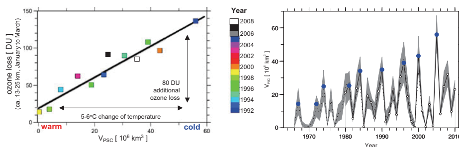
Fig. 11 Polar stratospheric clouds (PSC). Left PSC enhance stratospheric ozone loss (Harris et al. 2008). Right The volume of PSC estimated from meteorological analyses ( full line ECMWF; dashed line FU Berlin) has increased in the cold stratospheric winters, but not the warm ones (WMO 2011)
