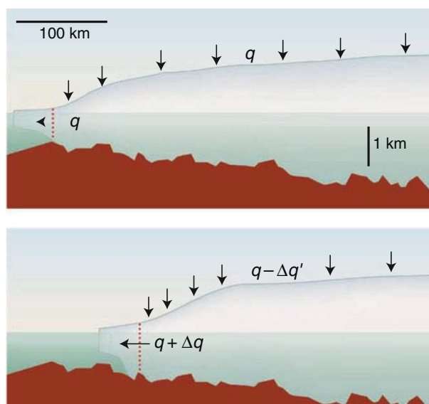
Fig. 5 Tipping of the West Antarctic Ice Sheet (WAIS). Possible self-amplification process of WAIS discharge (schematic from Vaughan and Arthern 2007). For regions in which the ice sheet is grounded below sea level ice flow across the grounding line (dashed vertical line) grows with ice thickness. If the bed is sloping down, ice discharge may self-accelerate
