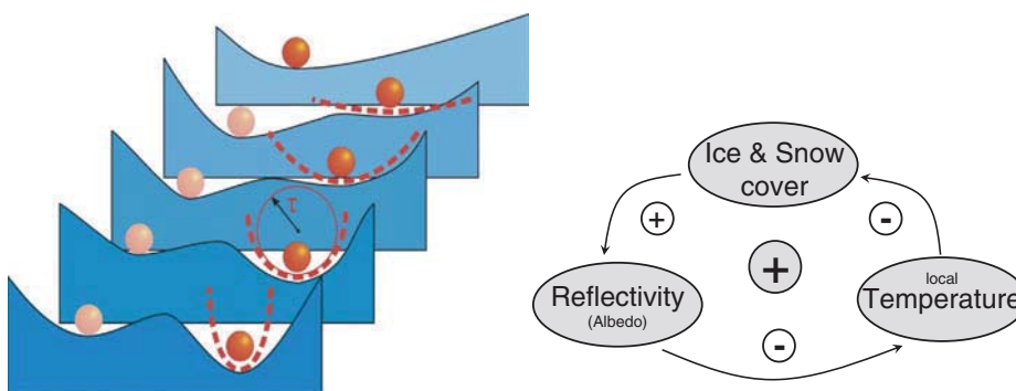
Fig. 2 Left Schematic illustrating the tipping of a system (Lenton et al. 2008). Initially (front), the system (dark orange ball) is stable within its background climate (blue valley). Initial changes in background climate do not alter the ball's position (or system's state). At a certain threshold small changes cause the ball to roll over. The system is tipping into a qualitatively different state. Right The ice-albedo feedback as an example of self-amplification which is at the heart of most tipping elements. A plus between two processes denotes an enhancing influence; a minus denotes reduction. For example, increased temperature reduces ice cover. An even number of minuses yields a self-amplification loop (denoted by '+' in the center of the loop)
