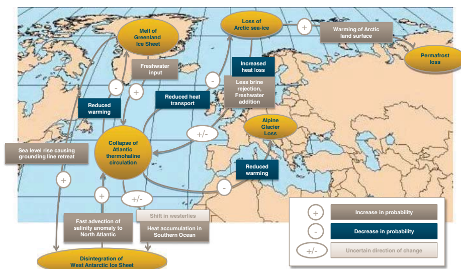
Fig. 13 Potential linkages between tipping elements
