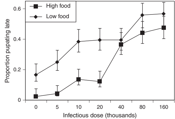
Figure 2 The effect of Vavraia culicis infectious dose and the mosquito's nutritional status on the proportion of Anopheles gambiae larvae pupating at least 8 days after hatching. Data points are presented as the mean \pm standard error of the proportion; diamonds represent mosquitoes reared on low food, squares mosquitoes reared on high food.
