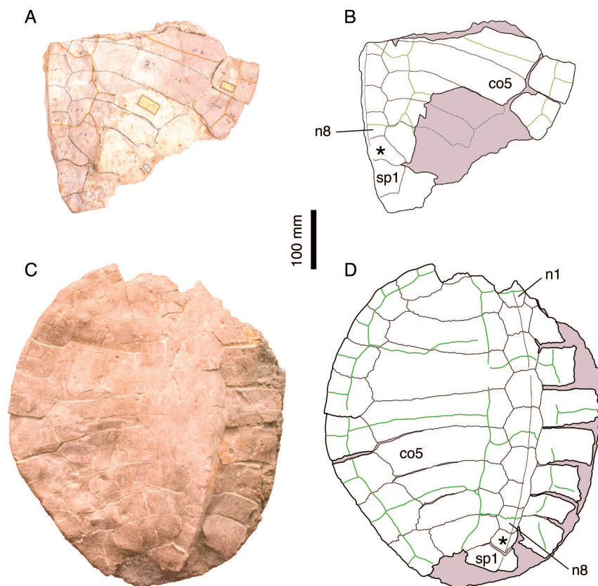
Figure 5 Tropicemys langii . Lectotype of Tr. langii , NMS 16: (A) photograph of the carapace; (B) interpretative drawing of the carapace. Referred specimen, NMS 15: (C) photograph of the carapace; (D) interpretative drawing of the carapace. Bones are white; green solid lines indicate scales sulci; matrix is gray. Abbreviations: co, costal; n, neural; sp, suprapygal; *, intermediate element (see text).
