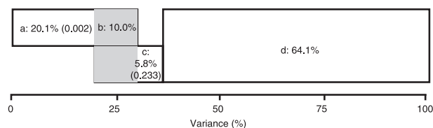
Fig. 3 Proportion of variance explained by phenotypic parameters, the phylogeny, both or neither, as established by a PVR analysis. Fraction a is linked only to phenotypic parameters; fraction b is linked both to phenotypic parameters and phylogeny; fraction c is linked only to the phylogeny; fraction d is the unexplained variance. The proportion of variance follows the letter which identifies each portion ( a-d ), followed, in parentheses (when this can be computed) by the associated probability.
