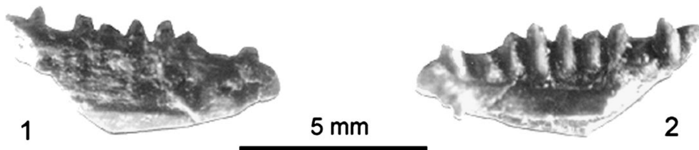
FIGURE 7—Right dentary of Slavoia cf. darevskii (KGE-Sh 10/1) from the Santonian-Campanian Bostobe Formation at Shakh-Shakh, Kazakhstan in buccal (1) and lingual (2) views.
