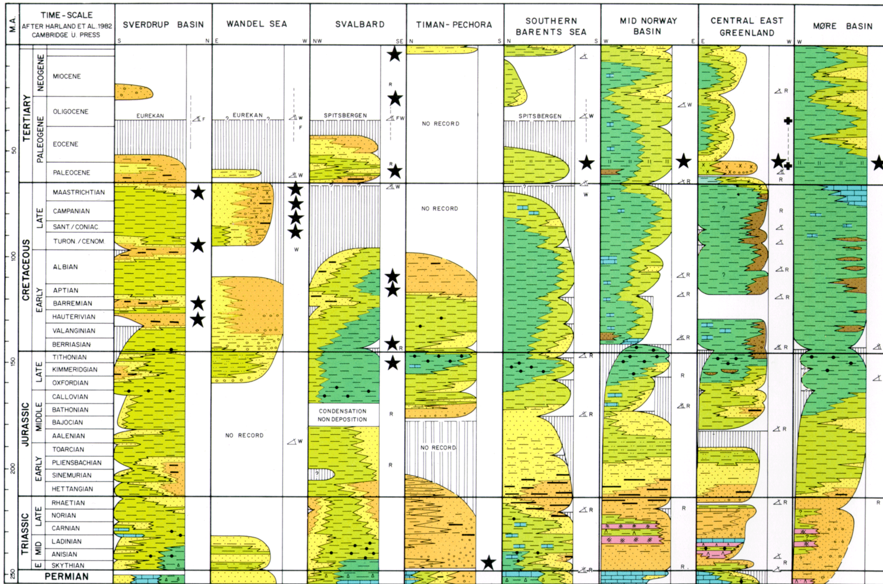
MESOZOIC AND CENOZOIC BASINS, ARCTIC AND NORWEGIAN-GREENLAND SEA
