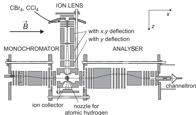
Figure 3. Schematic diagram of the instrument. Electron and ion beams are indicated by dashed lines. The monochromator is used only for diagnostic purposes and not while recording associative detachment spectra.
