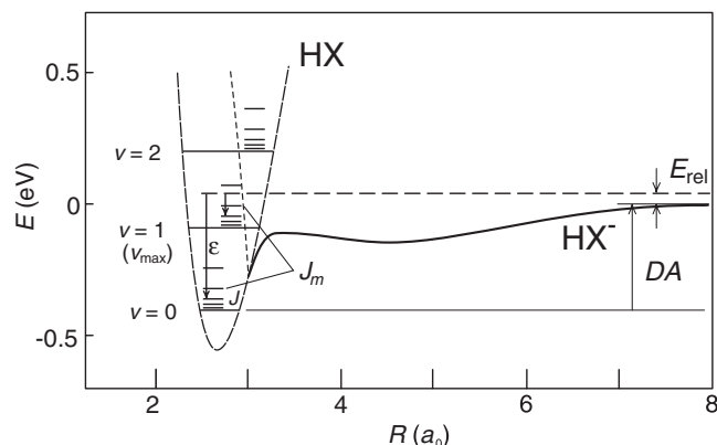
Figure 1. Schematic diagram of potential curves relevant for associative detachment, corresponding approximately to the \text{H} + \text{Br}^- case. E_{\text{rel}} is the CMS collision energy and DA the threshold energy for dissociative attachment. Two competing transitions into two different final vibrational but the same final rotational levels are indicated by vertical arrows. The separation of the rotational levels is shown exaggerated for clarity.
